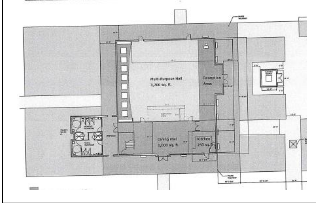
The original open-air temple concept and plan 2006
